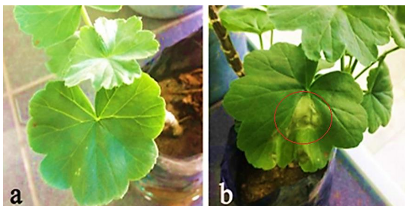
Fig. 2- Hypersensitivity reaction on geranium leaves, a) Negative control, b) Leaves inoculated with pathogenic strains isolated from apricot trees
